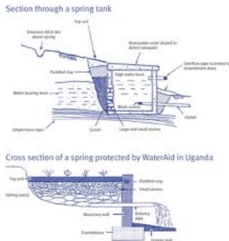
Figure 4.3. Example of Spring Protection from a WaterAID project in Uganda [15]
