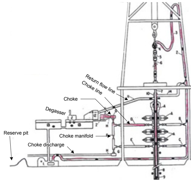
Figure 4-21: Killing operation during UBD (Rehm et al., 2007).
