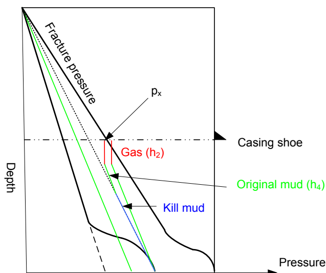
Figure 4-12: Comparing critical annular pressure for Driller's and Engineer's Method.
