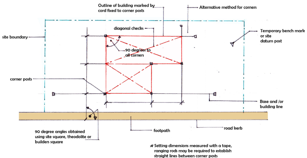
Figure 47: Setting out the Building
