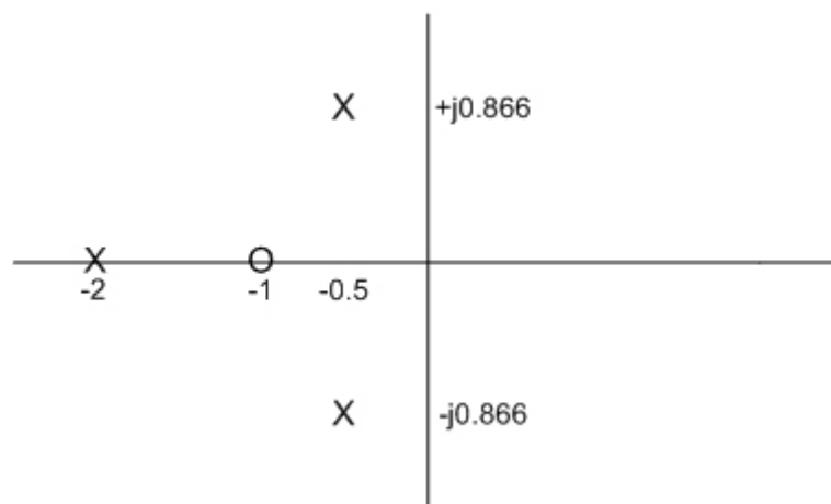
Figure 2.1 Zero-pole plot.
