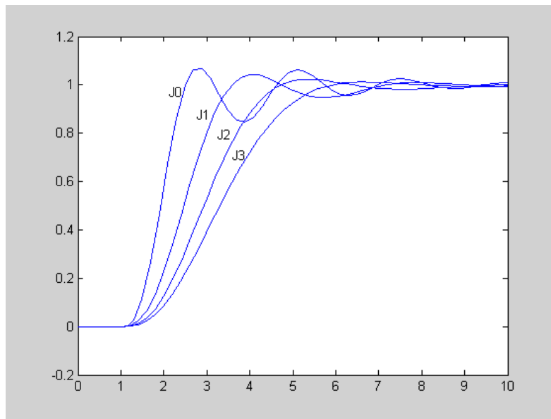
Figure 9.3 Response to a unit step at unit time for the standard form designs.
