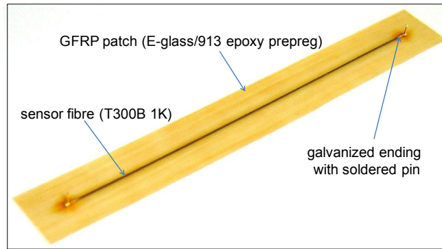
Figure 5.23 Carbon fibre sensor with an ex-Pan sensor fibre and a GFRP patch (source: Horoschenkoff & Christner 2012)
