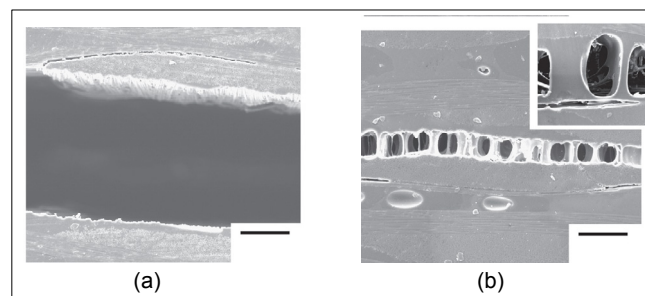
Figure 5.26 Scanning electron microscopy images of the delamination crack in a mendable laminate (a) before self-healing and (b) after self-healing. The inset photograph in (b) shows a higher magnification view of the crack bridging ligaments. Note the absence and presence of crack bridging ligaments of EMAA before and after healing, respectively (source: Pingkarawat et al. 2012)
