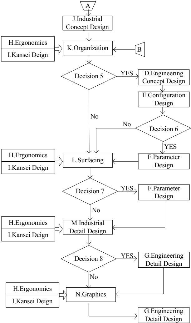
Fig. 7. Original design and redesign processes for a user-driven product
