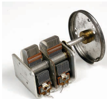
A variable air-gap capacitor such as those used in the tuning circuits of old radios. The semicircular plates rotate through the fixed plates, which changes the amount of surface area between the plates, and hence the capacitance. ( Loren Winters/Visuals Unlimited. )
