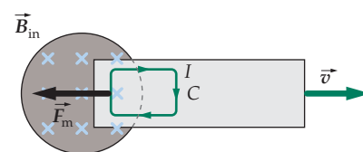
FIGURE 28-25 Demonstration of eddy currents. When the metal sheet is pulled to the right, there is a magnetic force to the left on the induced current opposing the motion.
