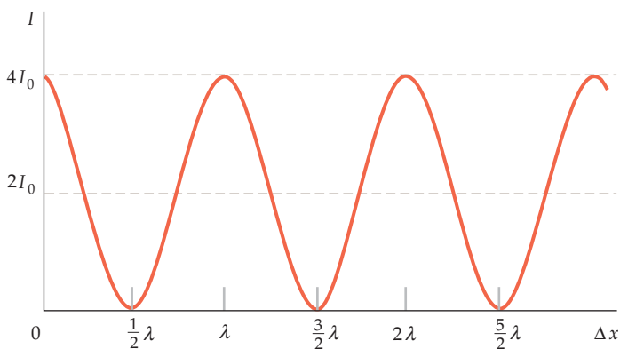
FIGURE 16-11 Intensity versus path difference for two sources that are in phase. I_0 is the intensity due to each source individually.
