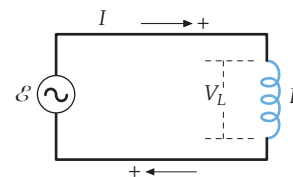
FIGURE 29-6 (repeated) An ac generator in series with an inductor L . The arrow indicates the positive direction along the wire. Note that for a positive value of dI/dt , the potential drop V_L across the inductor is positive.
