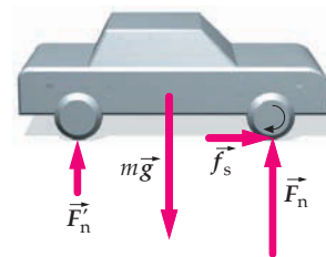
FIGURE 5-17 Forces acting on a car with front-wheel drive that is accelerating from rest. The normal force \vec{F}_n on the front tires is usually larger than the normal force \vec{F}'_n on the rear tires because typically the engine of the car is mounted near the front of the car. There is no drag force from the air shown because the car is just starting to move. There would be a rearward-directed rolling frictional force on all wheels, but that force has been ignored.
