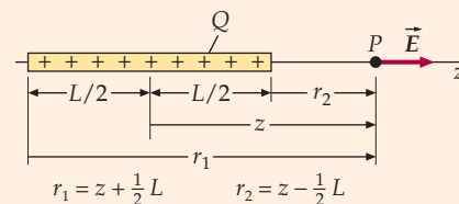
FIGURE 22-4 Geometry for the calculation of the electric field on the axis of a uniform line charge of length L , charge Q , and linear charge density \lambda = Q/L .
