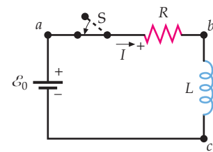
FIGURE 28-29 Just after the switch S is closed in this circuit, the current begins to increase and a back emf of magnitude L di/dt is induced in the inductor. The potential drop across the resistor IR plus the potential drop across the inductor ( L di/dt ) equals the emf of the battery ( \mathcal{E}_0 ).
