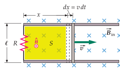
FIGURE 28-19 A conducting rod sliding on conducting rails in a magnetic field. As the rod moves to the right, the area of the surface S increases, so the magnetic flux through S into the paper increases. An emf of magnitude B\ell v is induced in the circuit, inducing a counterclockwise current that produces flux through the surface S directed out of the paper opposing the change in flux due to the motion of the rod.
