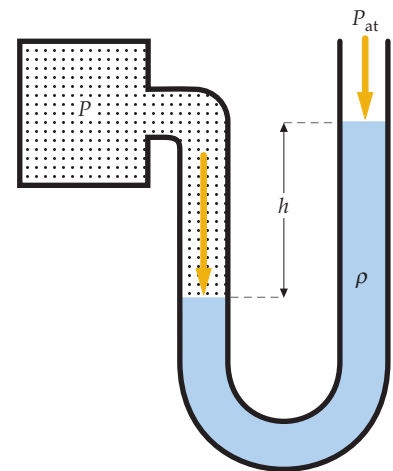
FIGURE 13-7 Open-tube manometer for measuring an unknown pressure P . The difference P - P_{\text{at}} equals \rho gh .
