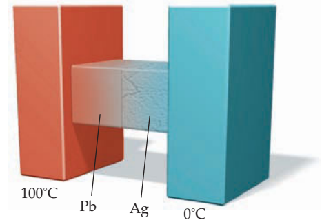
FIGURE 20-10 Two thermally conducting slabs of different materials in parallel.
