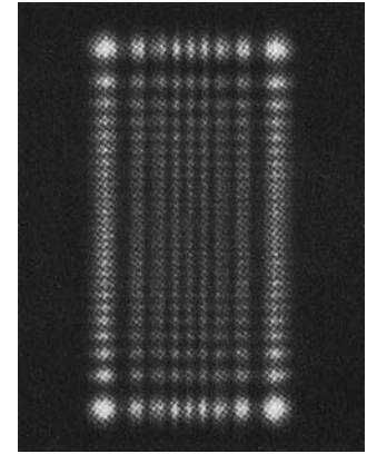
FIGURE 33-32 The Fresnel diffraction pattern of a rectangular aperture. (Courtesy of Michael Cagnet.)
