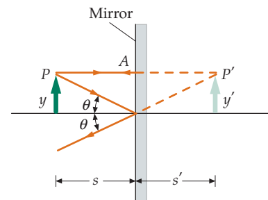
FIGURE 32-5 Ray diagram for locating the image of an arrow in a plane mirror.
