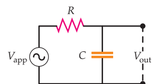
FIGURE 29-23 The peak output voltage decreases as frequency increases.
