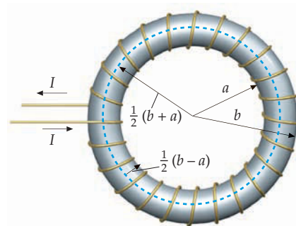
FIGURE 27-33 The toroid has mean radius r = \frac{1}{2}(b + a) , where a and b are the inner and outer radii of the toroid. Each turn of the wire is a circle of radius \frac{1}{2}(b - a) .
