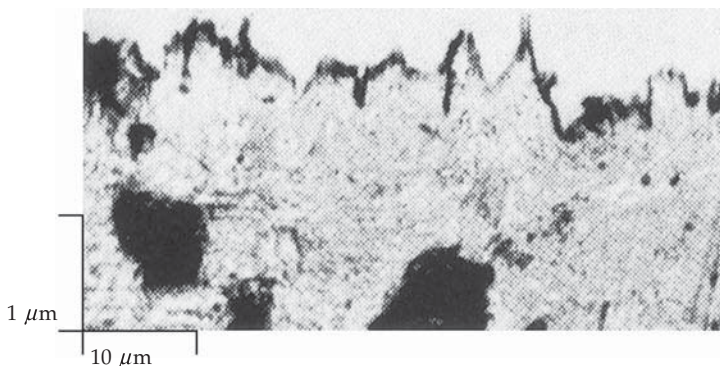
Magnified section of a polished steel surface showing surface irregularities. The irregularities are about = 5 \times 10^{-7} m high, a height that corresponds to several thousand atomic diameters. (From F. P. Bowden and D. Tabor, Lubrication of Solids , Oxford University Press, 2000.)
