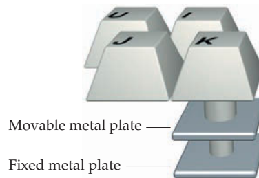
FIGURE 24-7 Capacitance switching in computer keyboards. A metal plate attached to each key acts as the top plate of a capacitor. Depressing the key decreases the separation between the top and bottom plates and increases the capacitance, which triggers the electronic circuitry of the computer to acknowledge the keystroke.
