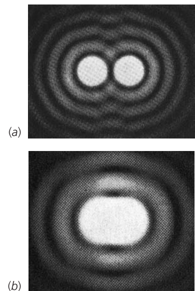
FIGURE 33-35 The diffraction patterns for a circular aperture and two incoherent point sources when (a) \alpha is a factor of 2 or so greater than \alpha_c = 1.22\lambda/D and (b) when \alpha is equal to the limit of resolution, \alpha_c = 1.22\lambda/D . ((a) and (b) Courtesy of Michael Cagnet.)
