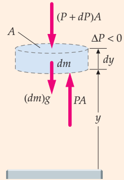
FIGURE 13-9 The pressure below the thin disk-shaped element of air is greater than the pressure above it. This pressure difference produces an upward force on the disk that balances the downward force of gravity on it.
