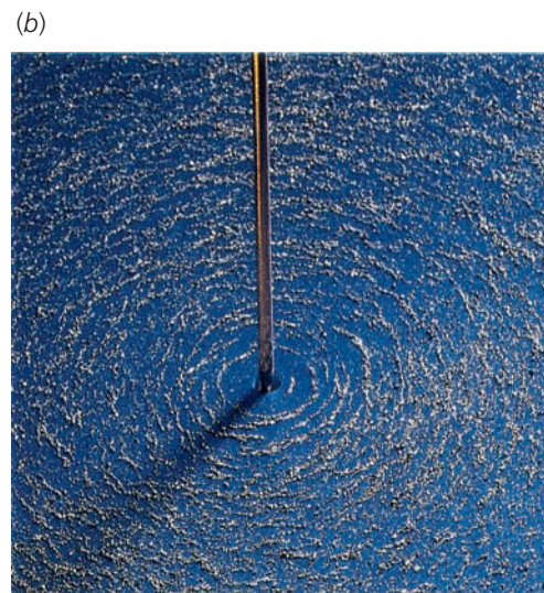
FIGURE 27-18 (a) Right-hand rule for determining the direction of the magnetic field due to a long, straight, current-carrying wire. The magnetic field lines encircle the wire in the direction of the fingers of the right hand when the thumb points in the direction of the current. (b) Magnetic field lines due to a long wire, which is indicated by iron filings. (© 1990 Richard Menga/Fundamental Photographs.)
