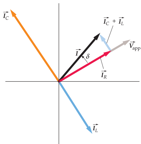
FIGURE 29-26 A phasor diagram for the currents in the parallel RLC circuit shown in Figure 29-25. The potential drop is the same across each element. The current in the resistor is in phase with the potential drop. The current in the capacitor leads the potential drop by 90^\circ and the current in the inductor lags the potential drop by 90^\circ . The phase difference \delta between the total current and the potential drop depends on the relative magnitudes of the currents, which depend on the values of the resistance and of the capacitive and inductive reactances.
